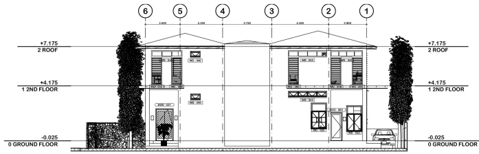
A3.1 REAR ELEVATION 1:150
