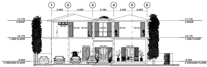
A3.1 FRONT ELEVATION 1:150
