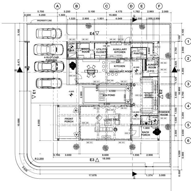
GROUND FLOOR PLAN 1:150
