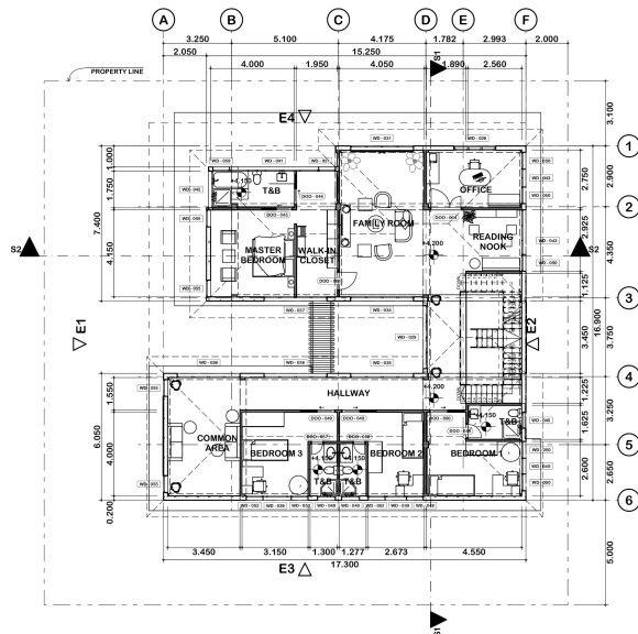
2ND FLOOR 1:150
