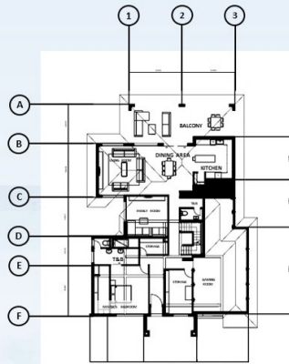
GROUND FLOOR PLAN SCALE: 1:500 MTS
