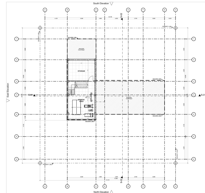
BASEMENT PLAN
