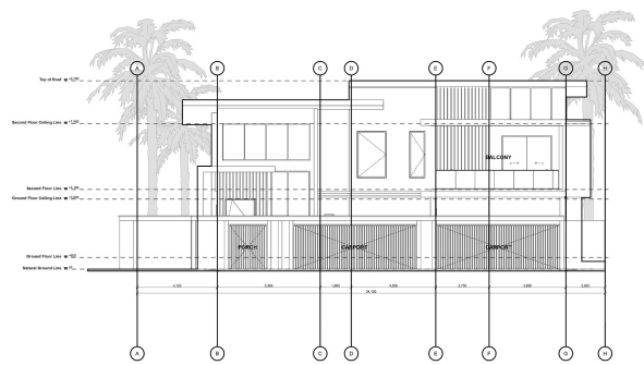
FRONT ELEVATION 1:150
