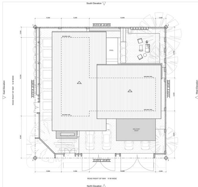
SITE DEVELOPMENT PLAN
