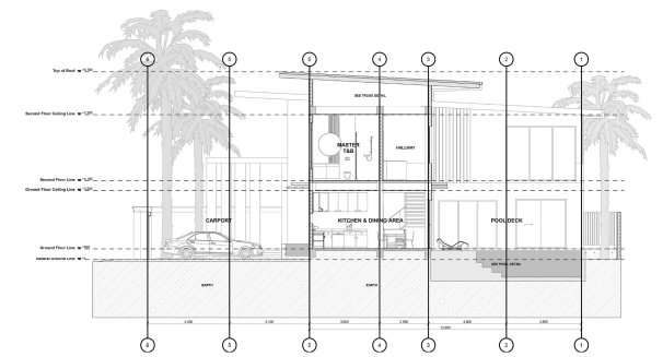
S-02 CROSS SECTION 1:150
