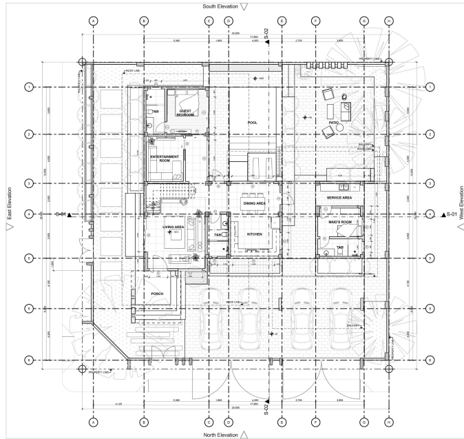
GROUND FLOOR PLAN 1:150
